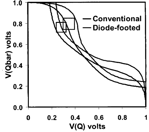
Figure 4. Static noise margin of diode-footed cache.
