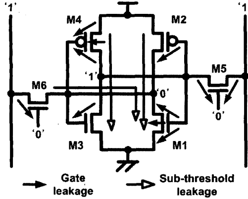
Figure 2. Dominant leakage components in a 6T SRAM.
