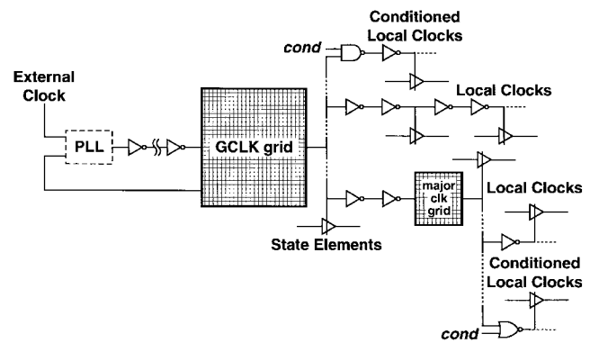
Fig. 1. Clock hierarchy.
