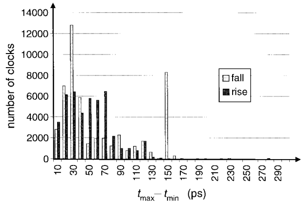
Fig. 10. Differences between minimum and maximum clock node delays.
