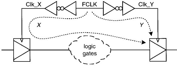
Fig. 7. Example circuit illustrating race-through and critical path constraints.
