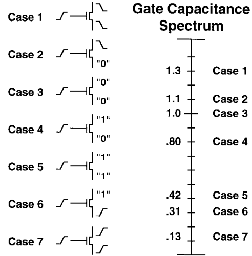
Fig. 8. Data-dependent gate loading.
