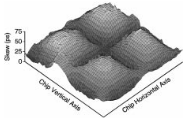
Fig. 4. Simulated global clock skew.
