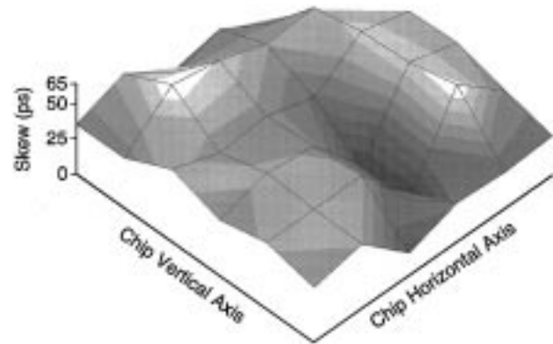
Fig. 5. Measured global clock skew.
