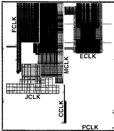
Fig. 6. Major clock grids.
