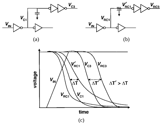
Fig. 9. Resistance isolation and downstream effects. (a) Example clock distribution network without resistance. (b) Example clock distribution network including resistance. (c) Waveforms.
