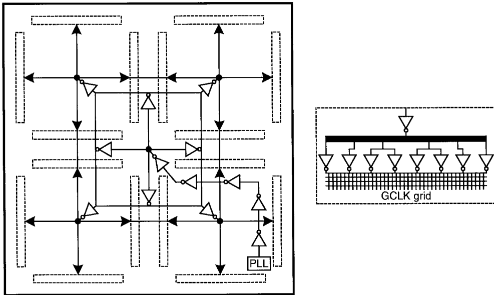
Fig. 2. Global clock distribution network.
