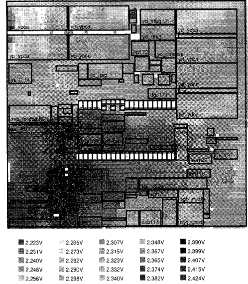
Figure 10: Vdd distribution without additional on-chip decoupling capacitors
