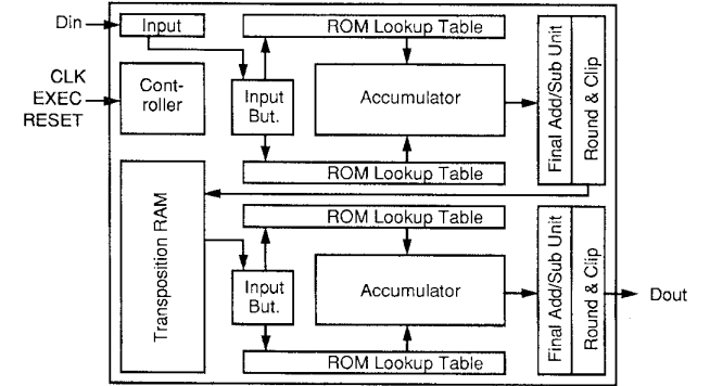
Fig. 9. DCT block diagram.
