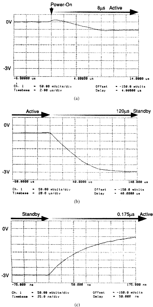
Fig. 13. Measured p-well V_{BB} : (a) after power-on, (b) active-to-standby, and (c) standby-to-active.
