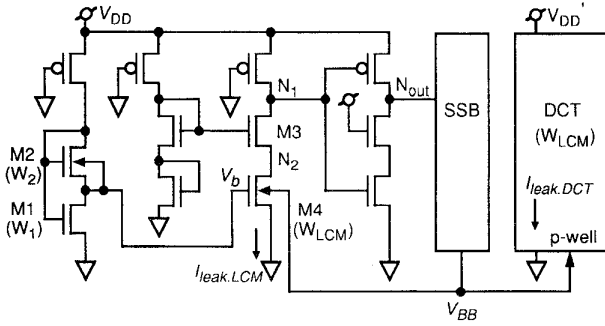
Fig. 5. Leakage current monitor (LCM).
