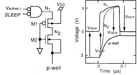
Fig. 8. SCI and its waveforms simulated by SPICE.
