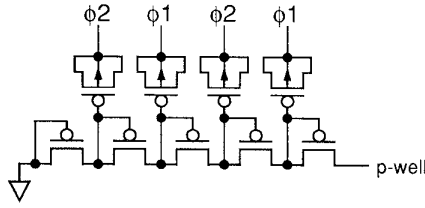
Fig. 7. Pump circuit in SSB.
