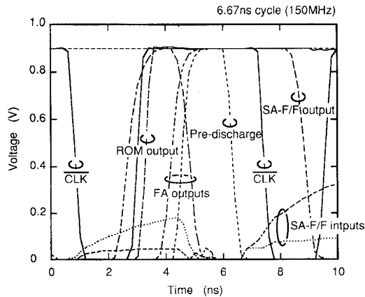
Fig. 10. Simulated waveforms of MAC datapath.
