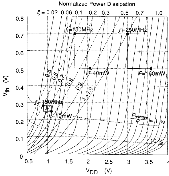
Fig. 1. Exploring low- V_{DD} , low- V_{th} design space. Contour lines in terms of speed (broken lines) and power (solid lines) are drawn.
