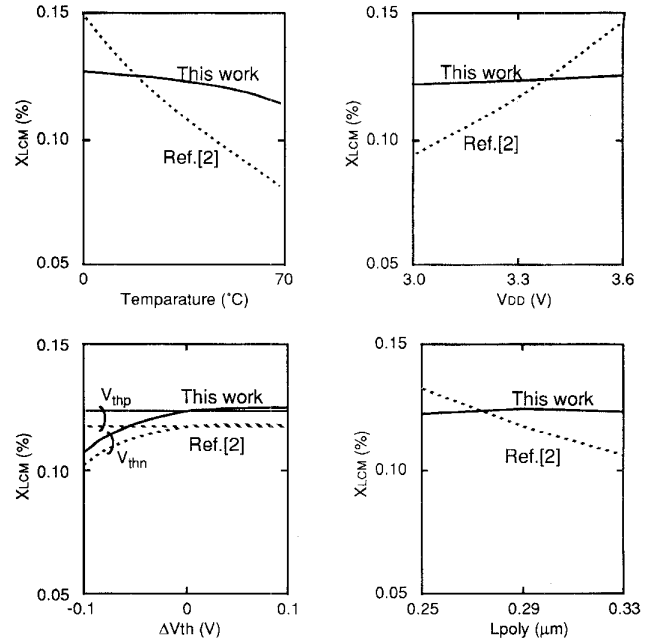
Fig. 6. Current magnification factor of the LCM, X_{\text{LCM}} , dependence on circuit condition changes and process deviations simulated by SPICE.
