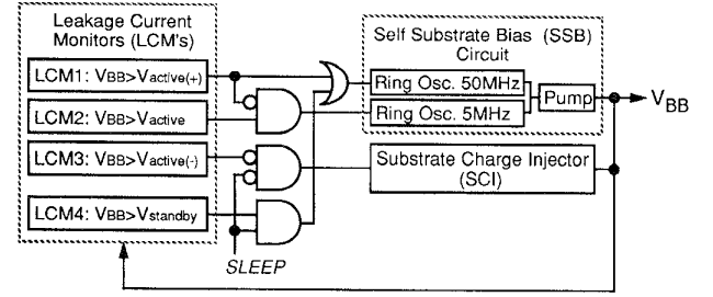
Fig. 3. VT block diagram.
