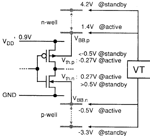
Fig. 2. Variable threshold-voltage (VT) scheme.
