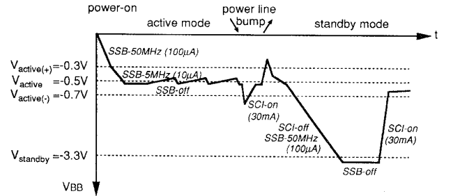
Fig. 4. Substrate-bias control in VT.
