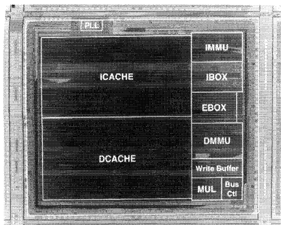
Fig. 1. Chip photo with overlay.
