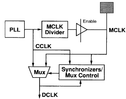
Fig. 10. Clock switching circuit.
