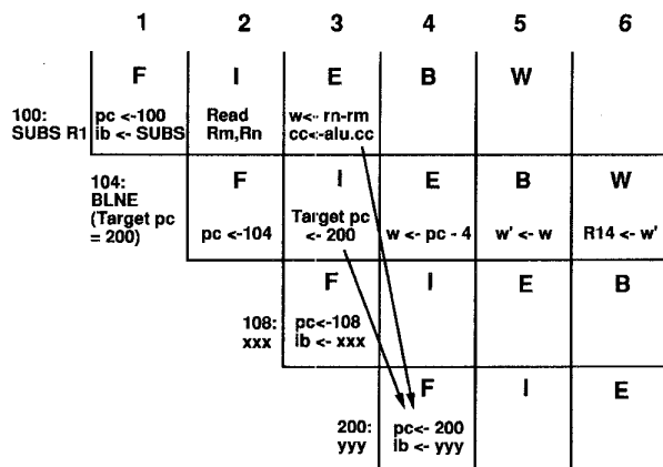
Fig. 3. Pipeline diagram of a branch.
