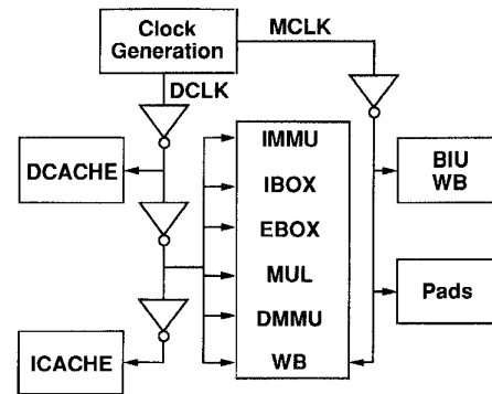
Fig. 7. Clock regimes.
