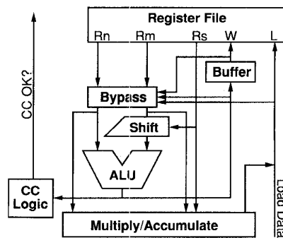
Fig. 4. EBOX block diagram.
