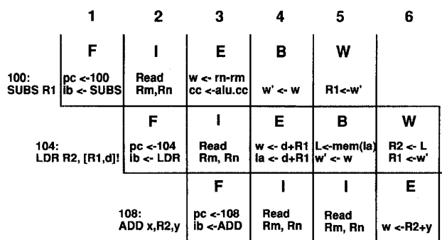
Fig. 2. Basic pipeline diagram.
