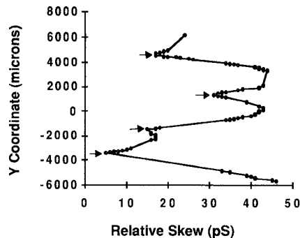
Fig. 9. Clock arrival time in the core.
