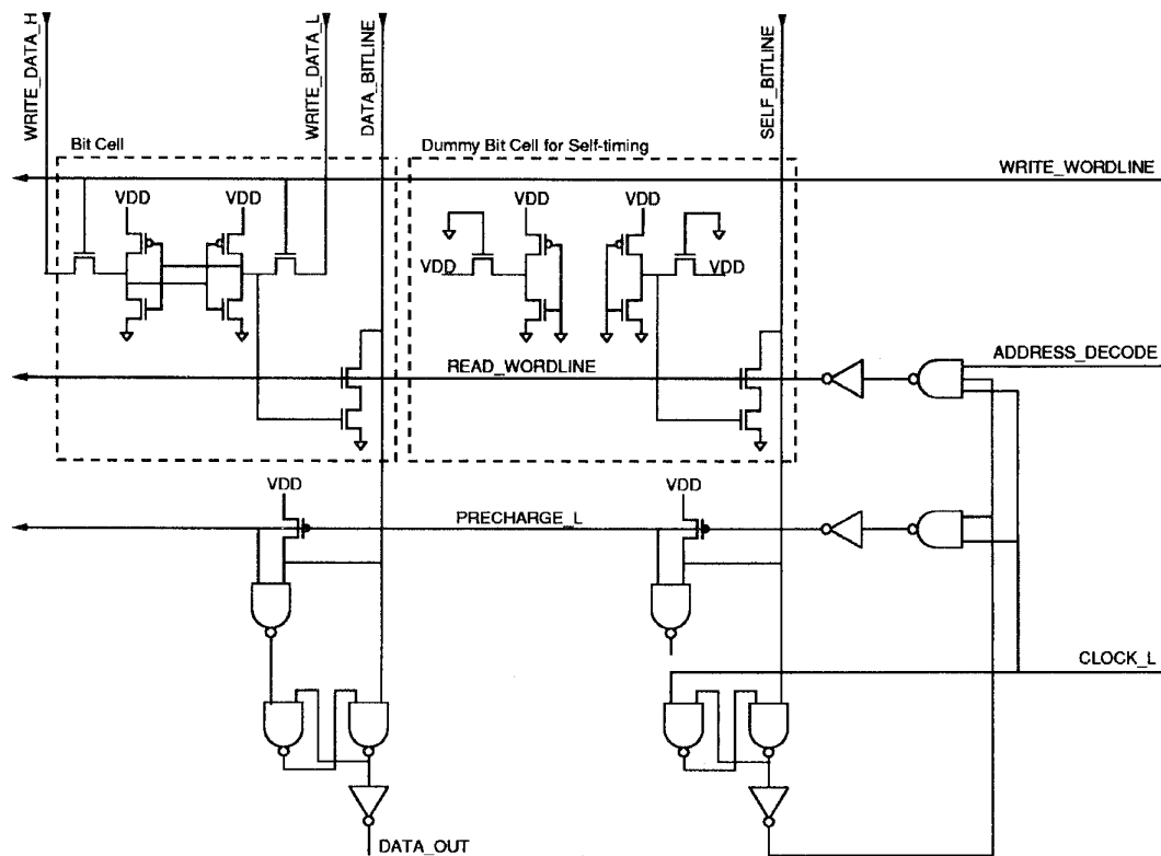
Fig. 6. Self-timed RF precharge.
