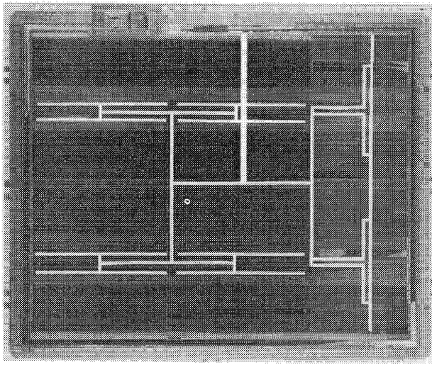
Fig. 8. Physical routing of clock tree.
