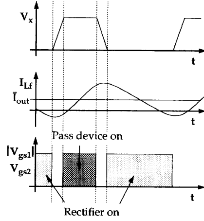
Fig. 2. Nominal waveforms of the buck circuit in Figure 1.
