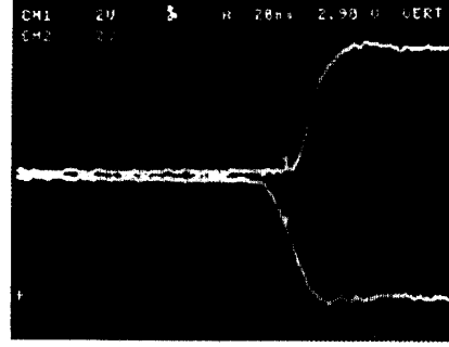
Fig. 6. A zero-voltage-switched high to low inverter transition. The vertical scale is 2 V/div; the horizontal scale is 20 ns/div.
