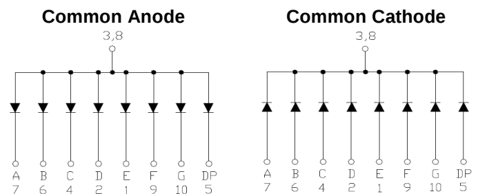
Figure 1. INND-TS56 series Internal Circuit Diagram
